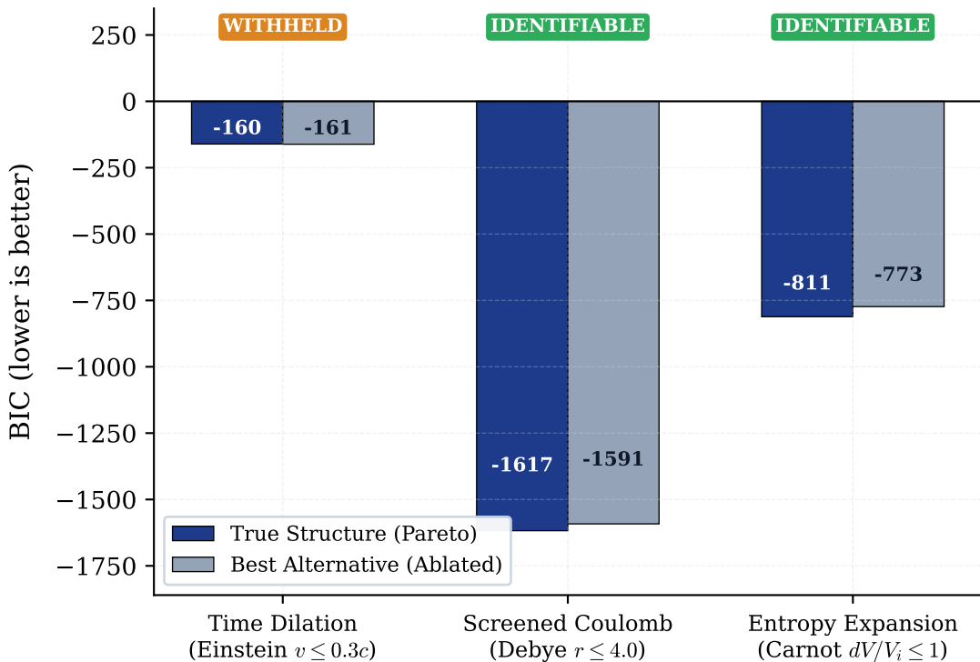
(a) Absolute BIC Model Selection
