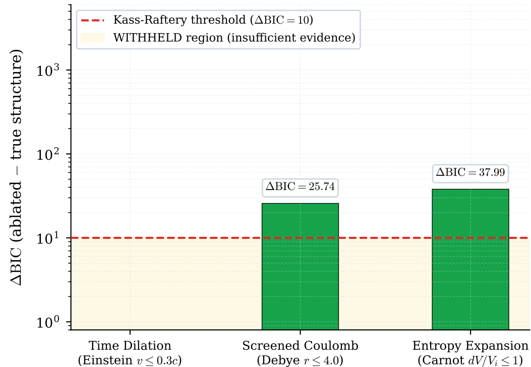
(b) Identifiability Evidence ( \Delta\text{BIC} )
