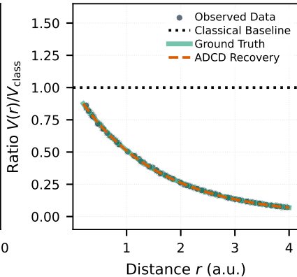
(b) Screened Coulomb Potential
