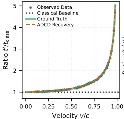
(a) Time Dilation
