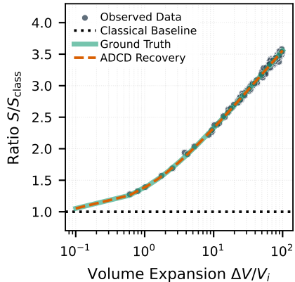
(c) Non-ideal Entropy
