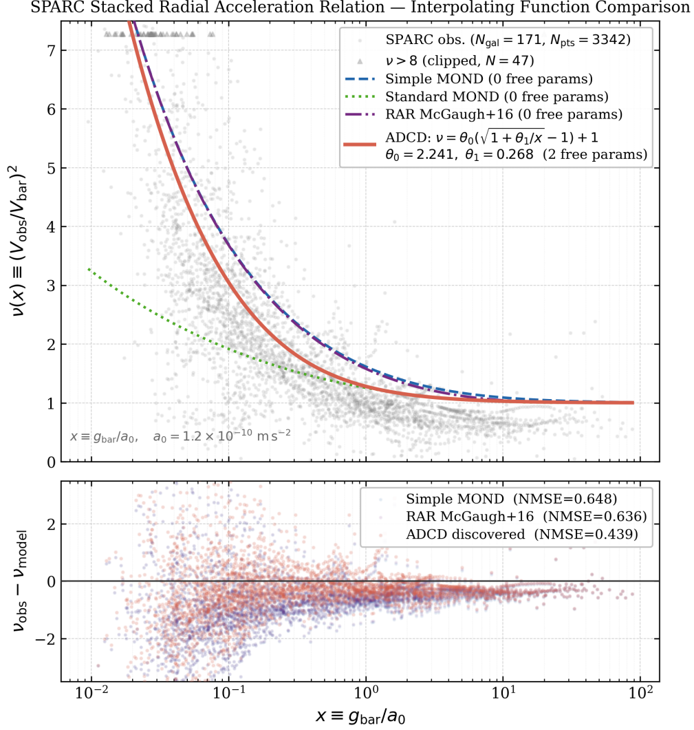
Figure 6: SPARC stacked radial acceleration relation. Upper: observed \nu(x) (grey) against the four interpolating functions. The AD CD-discovered 2-parameter curve (red) tracks the data more tightly than Simple/Standard MOND and the McGaugh+16 RAR form. Lower: residuals \nu_{\text{obs}} - \nu_{\text{model}} .
