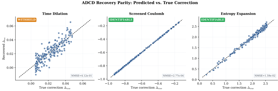
Figure 3: Parity plots: recovered correction ( \Delta_{\text{rec}} ) vs. true correction ( \Delta_{\text{true}} ) for N = 200 data points. Black dashed: 1:1 reference line. The near-perfect diagonal for Screened Coulomb ( \text{NMSE} = 2.77 \times 10^{-4} ) illustrates a clean exact match achieved without any symbolic hint of the solution. Scatter for Time Dilation ( \text{NMSE} = 0.41 ) reflects the insufficient signal-to-noise ratio at v \leq 0.3c .
