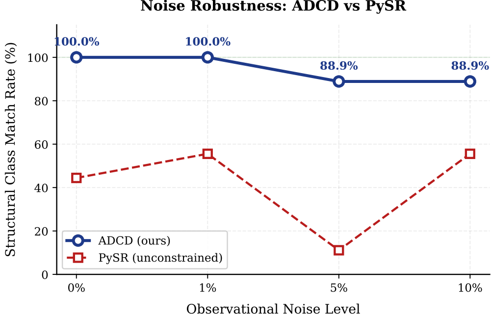
Figure 2: Structural class match rate as a function of observational noise level. ADCD (Mock Proposer, seed=42) maintains 88.9% structural accuracy at 5% noise due to physics-constrained gate filtering. PySR (fair profile, unconstrained SR on the same residual) exhibits a non-monotonic noise-accuracy profile (44.4%→55.6%→11.1%→55.6%), reflecting overfitting instabilities absent from physics-gated search.
