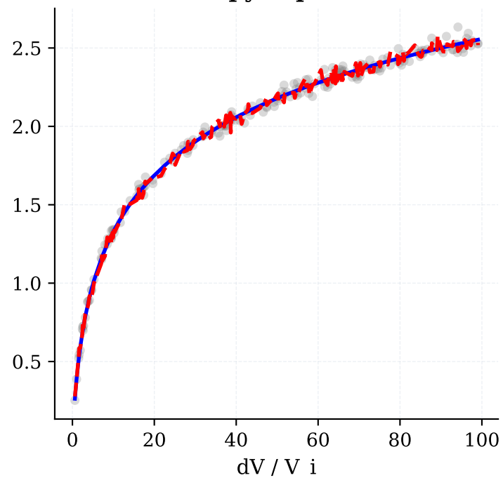
Entropy Expansion
