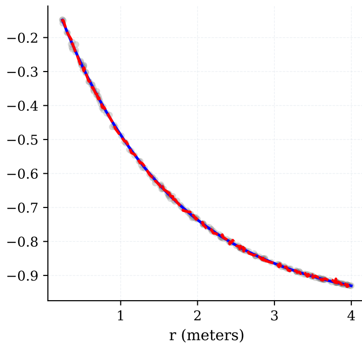
Screened Coulomb
