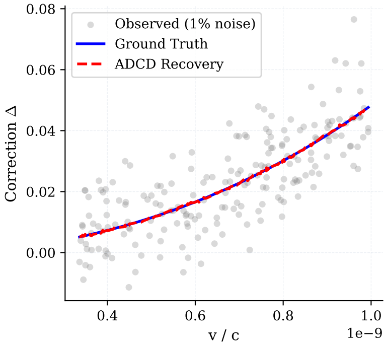
Time Dilation
