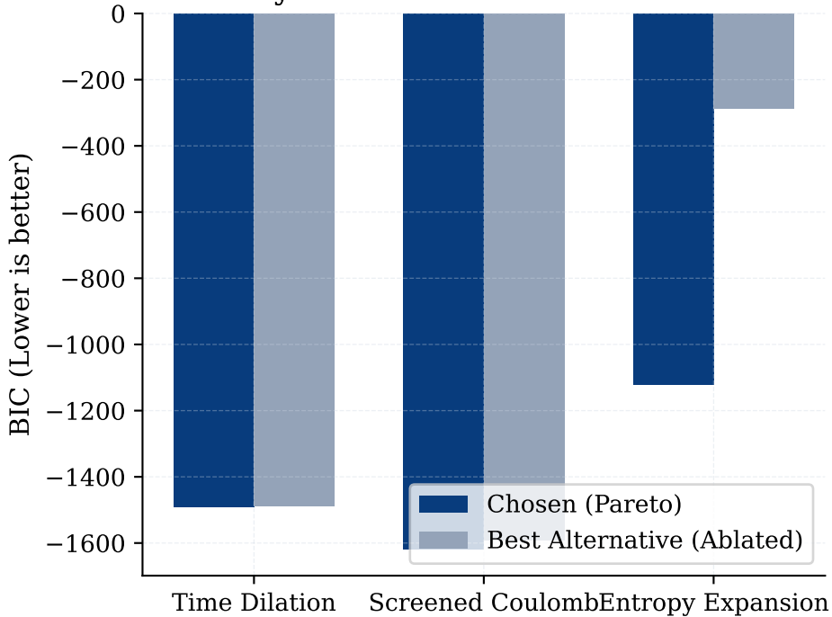
Bayesian Information Criterion
