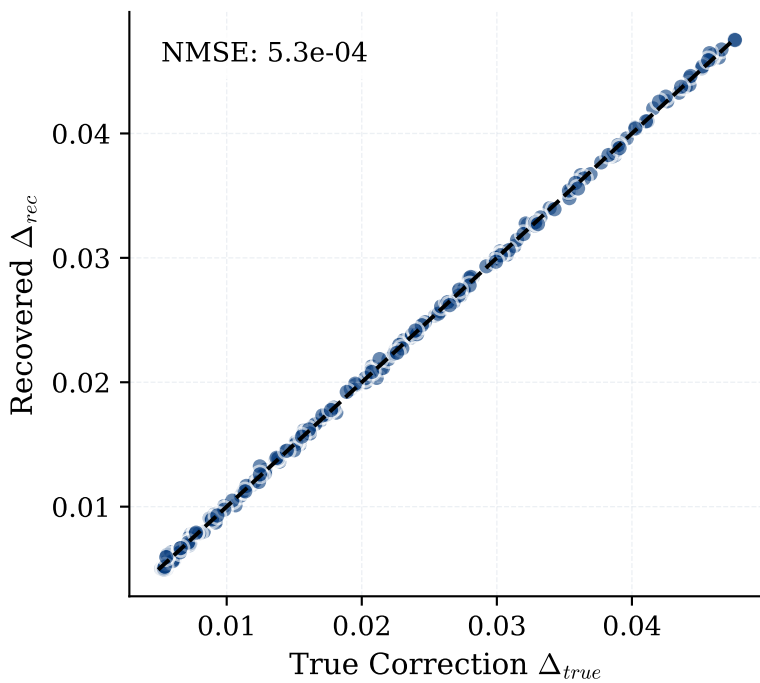
Time Dilation
