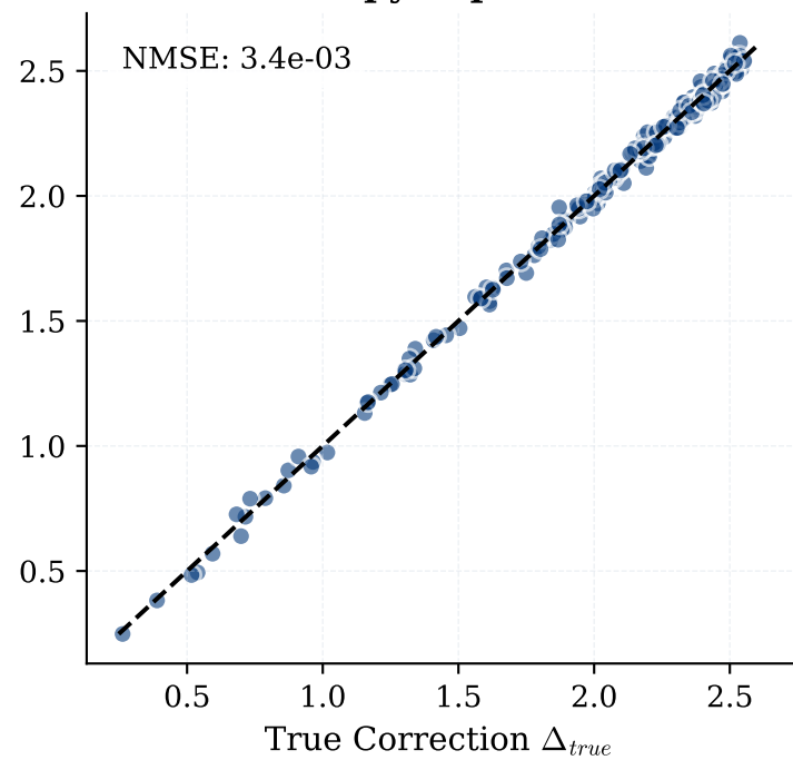
Entropy Expansion
