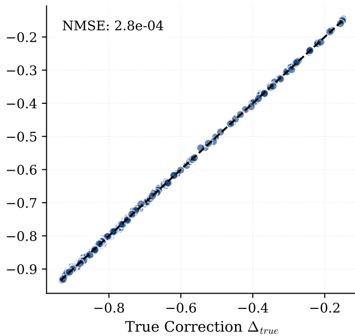
Screened Coulomb
