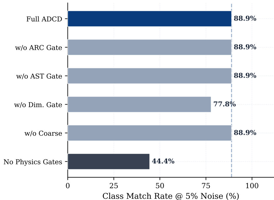
(b) Gate Contribution (Ablation)
