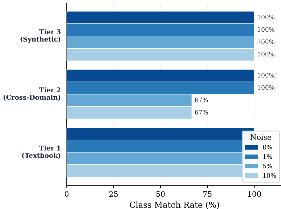
(a) Accuracy by Tier & Noise
