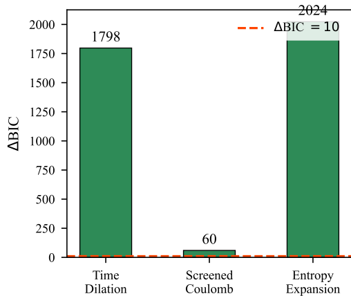
(b) Identifiability: \Delta BIC
