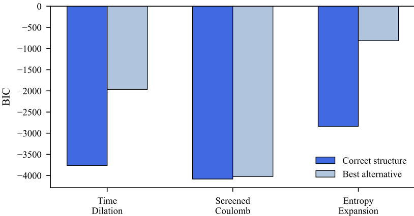
(a) BIC: Correct vs. Best Alternative
