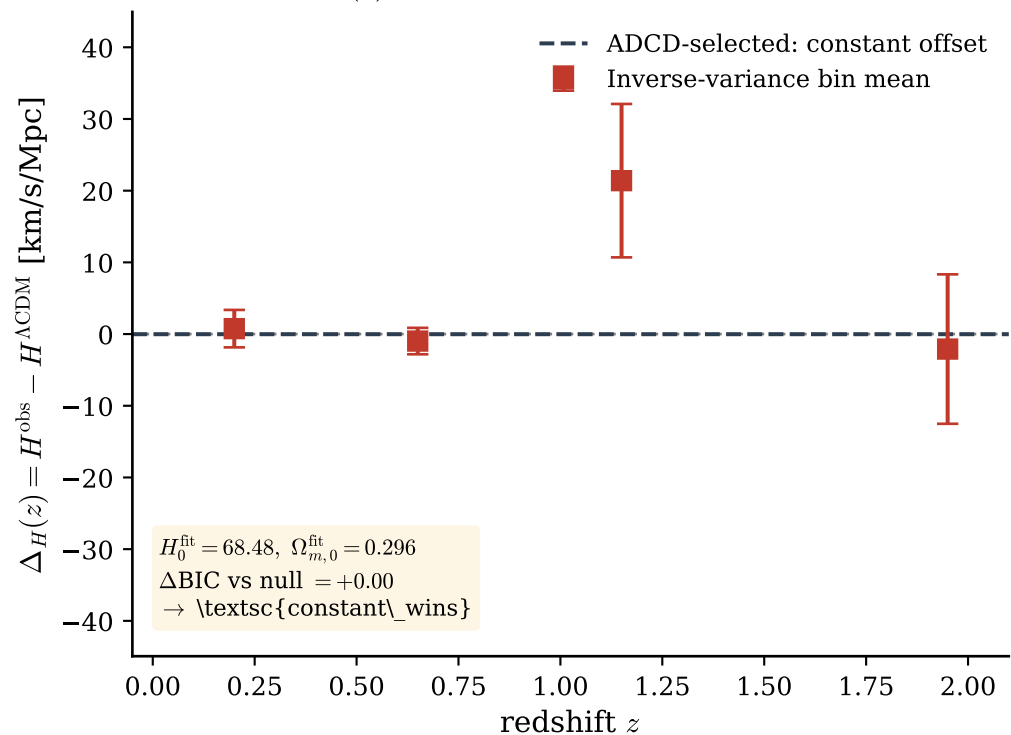
(b) H(z) cosmic chronometers ( N=34 )
