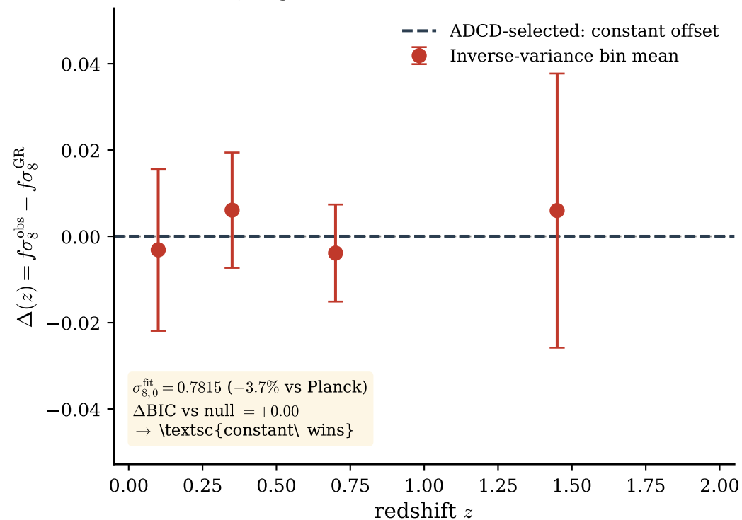
(a) f\sigma_8 growth rate ( N=63 , Alestas+22)
