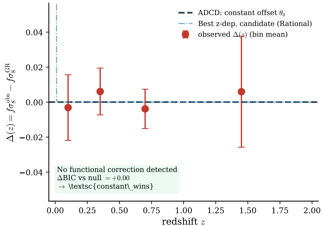
(b) Cosmological: f\sigma_8 — amplitude only
