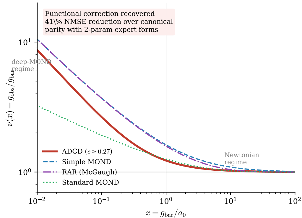
(a) Galactic: SPARC — functional recovery
