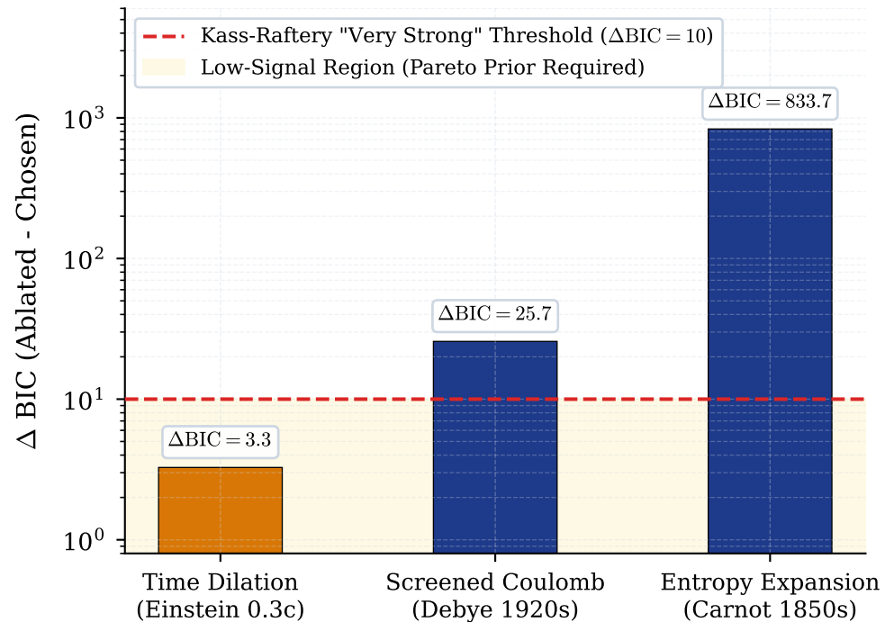
(b) Statistical Evidence Strength ( \Delta\text{BIC} )
