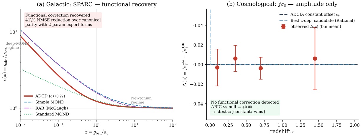
Figure 9: The structural dichotomy in one figure. (a) Galactic scale (SPARC): ADCD recovers a functional interpolating curve (red) that tracks the data across the Newtonian-to-deep-MOND transition, dominating the zero-parameter canonical MOND/RAR forms. (b) Cosmological scale ( f\sigma_8 ): the residual carries no z -dependent structure; ADCD selects a constant amplitude offset (dashed), and the best z -dependent candidate (Rational, dot-dashed) is statistically indistinguishable from it ( \Delta\text{BIC} = +0.42 , far below the decisive threshold). Individual gravitational systems admit functional corrections; large-scale cosmological tensions appear as amplitude offsets.
