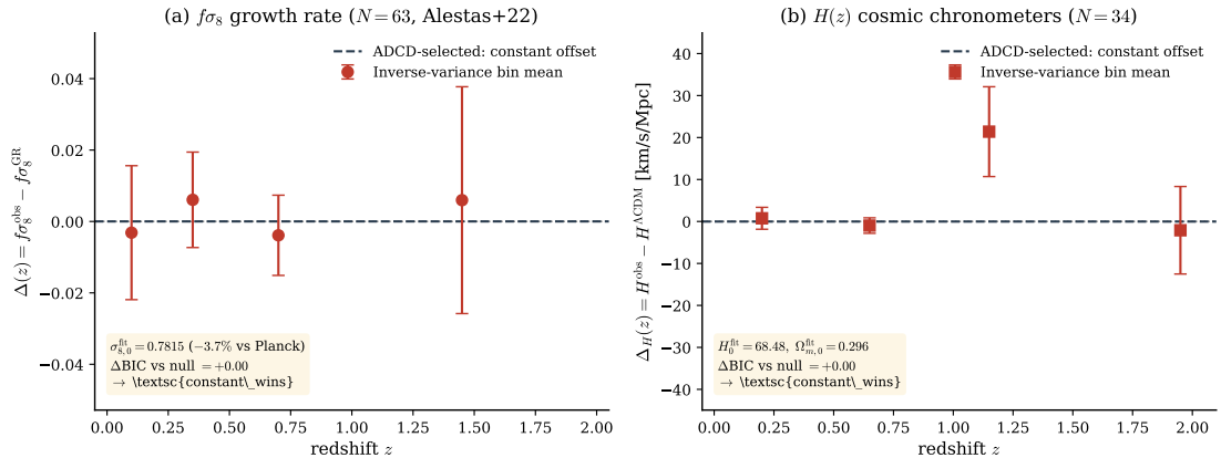
Figure 7: Cosmological-probe residuals and the CONSTANT_WINS verdict. (a) f\sigma_8 residual \Delta(z) = f\sigma_8^{\text{obs}} - f\sigma_8^{\text{GR}} (63 points, Alesta+22); the GR baseline has \sigma_{8,0} free. Inverse-variance bin means (red) are consistent with zero across all redshifts ( |\text{pull}| \leq 0.5\sigma ), and the ADCD-selected model is the 1-parameter constant offset (dashed). (b) Same for H(z) (34 cosmic-chronometer points); the best candidate is again the constant offset. In both observables no z -dependent functional form beats a pure amplitude rescaling by \Delta\text{BIC} < -10 .
