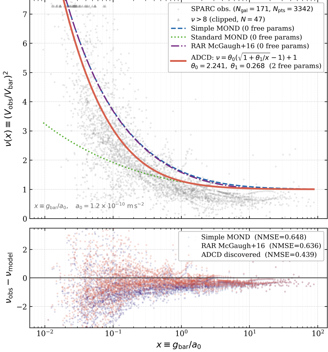
SPARC Stacked Radial Acceleration Relation — Interpolating Function Comparison
