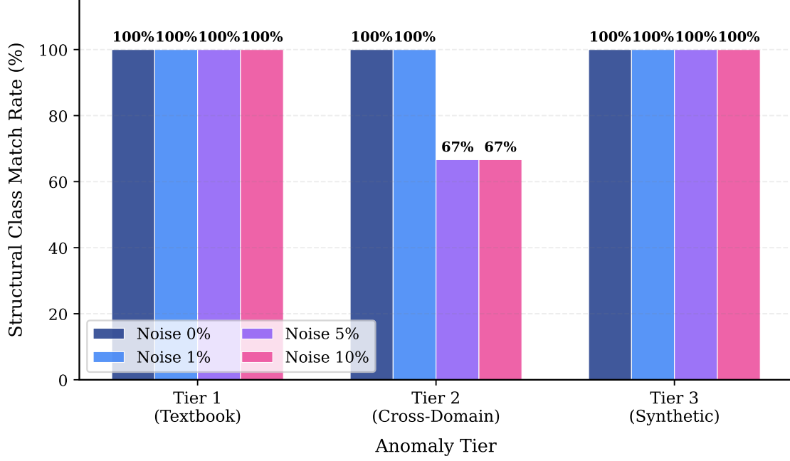
ADCD Performance by Tier and Noise Level
