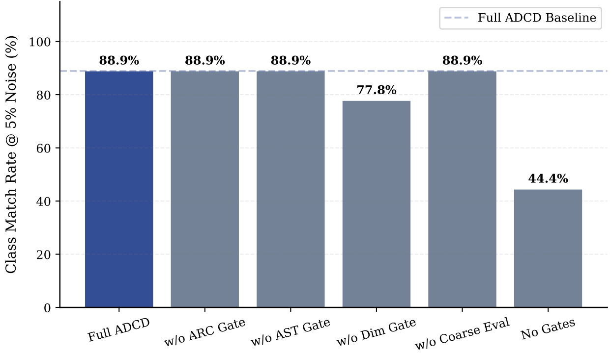
Figure 5: Ablation study at 5% observational noise. Each bar disables one gate. Removing the ARC, AST, or Coarse-Eval gate individually leaves structural accuracy unchanged (8/9). Removing the dimensional gate alone reduces accuracy by 11.1 pp (8/9 to 7/9). Only removing all gates simultaneously causes a larger collapse, dropping performance by \Delta = 44.5 percentage points (from 8/9 to 4/9), confirming that the gates reinforce each other as a collective physical consistency filter. Note: the “Without BIC Reranking” condition is described in Section 6 but excluded from this figure as it requires the full gate pipeline to isolate BIC’s contribution.
