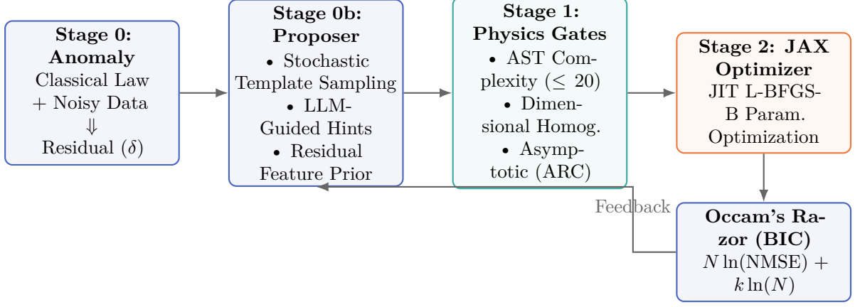
Figure 1: System architecture of the Anomaly-Driven Correction Discovery (ADCD) framework.
