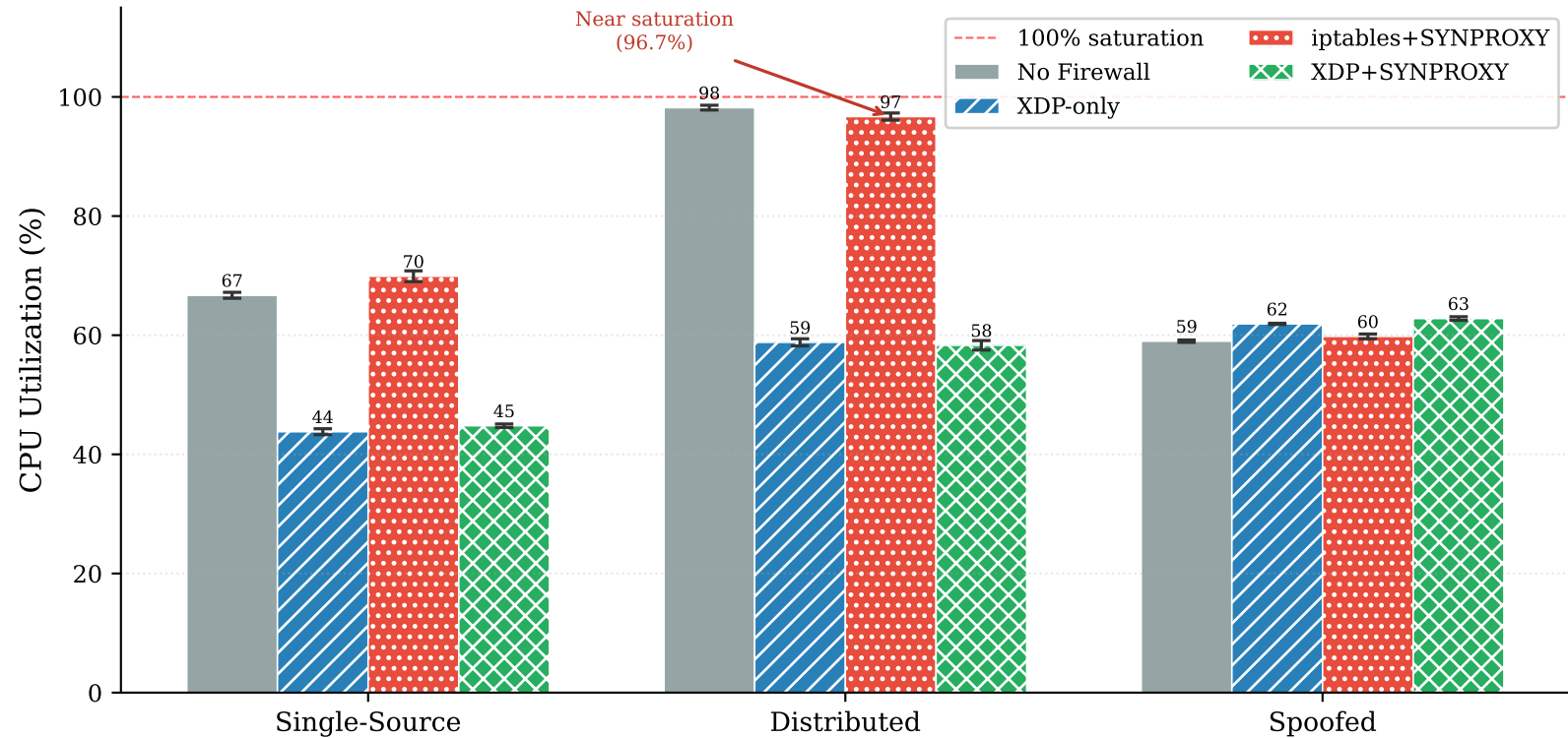
CPU Utilization — Emulated Testbed (50 kpps, mean \pm std, 3 runs, N = 120 per run)
