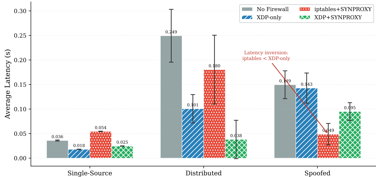
Average Latency — Emulated Testbed (50 kpps, mean \pm std, 3 runs, N = 120 per run)
