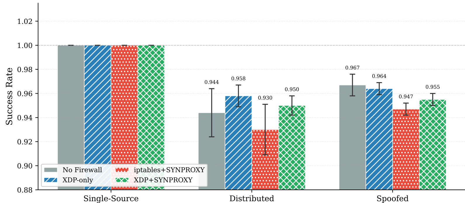
Service Success Rate — Emulated Testbed (50 kpps, mean \pm std, 3 runs, N = 120 per run)
