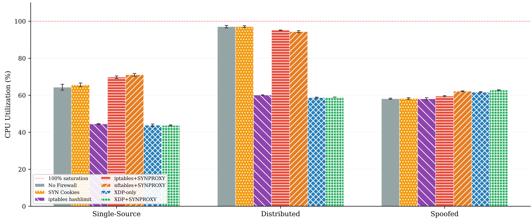
CPU Utilization (%) — 7 Mitigation Mechanisms (50 kpps, mean \pm std, 3 runs, N=120/run)
