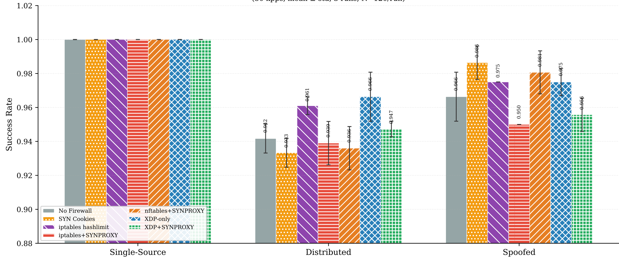
Success Rate — 7 Mitigation Mechanisms (50 kpps, mean \pm std, 3 runs, N=120/run)
