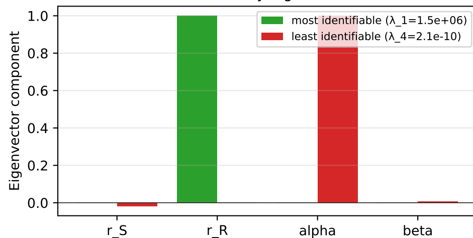
Identifiability eigenvectors
