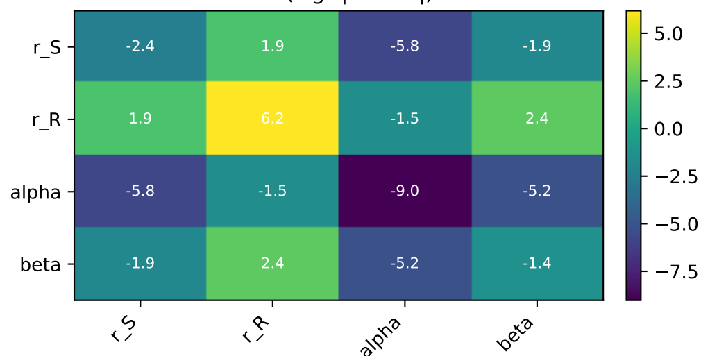
FIM ( \log_{10}|\text{entries}| )
