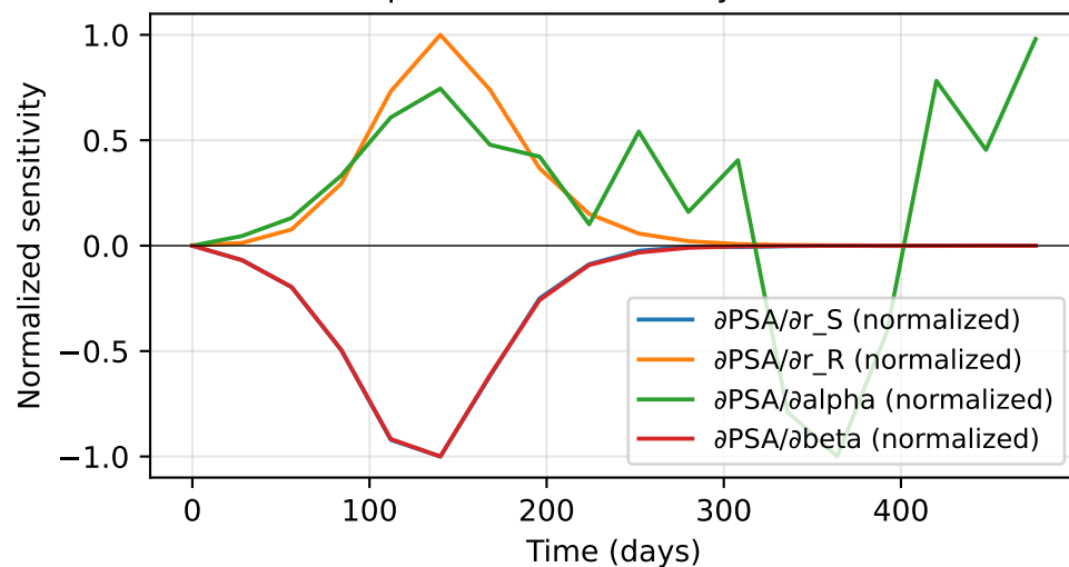
Per-parameter sensitivity over time
