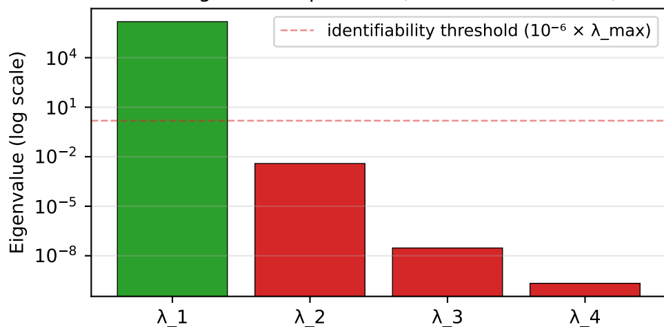
FIM eigenvalue spectrum (effective rank = 1/4)
