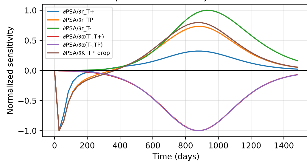
Per-parameter sensitivity over time
