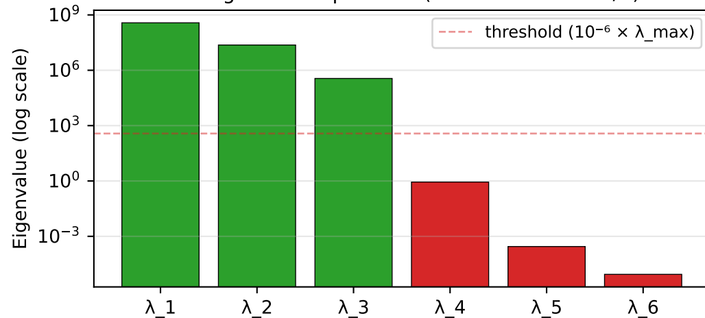
FIM eigenvalue spectrum (effective rank = 3/6)
