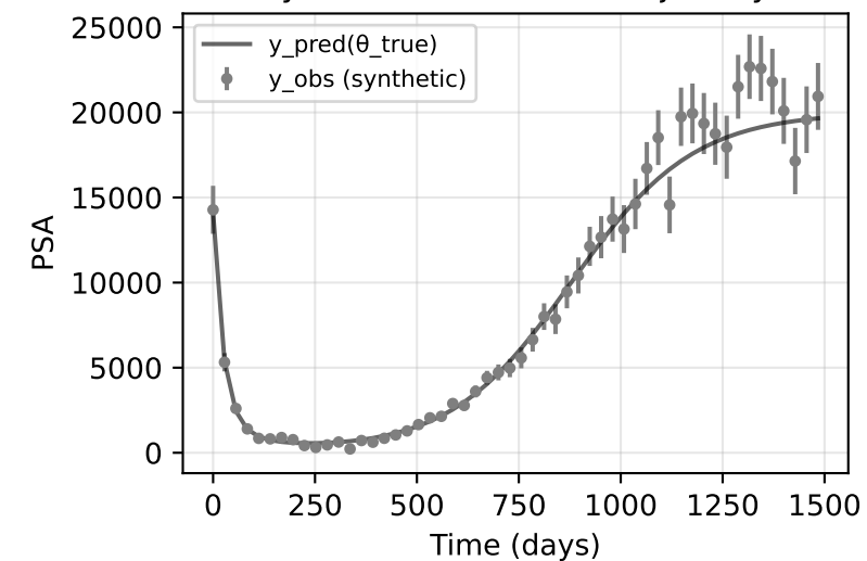
Synthetic data + true trajectory
