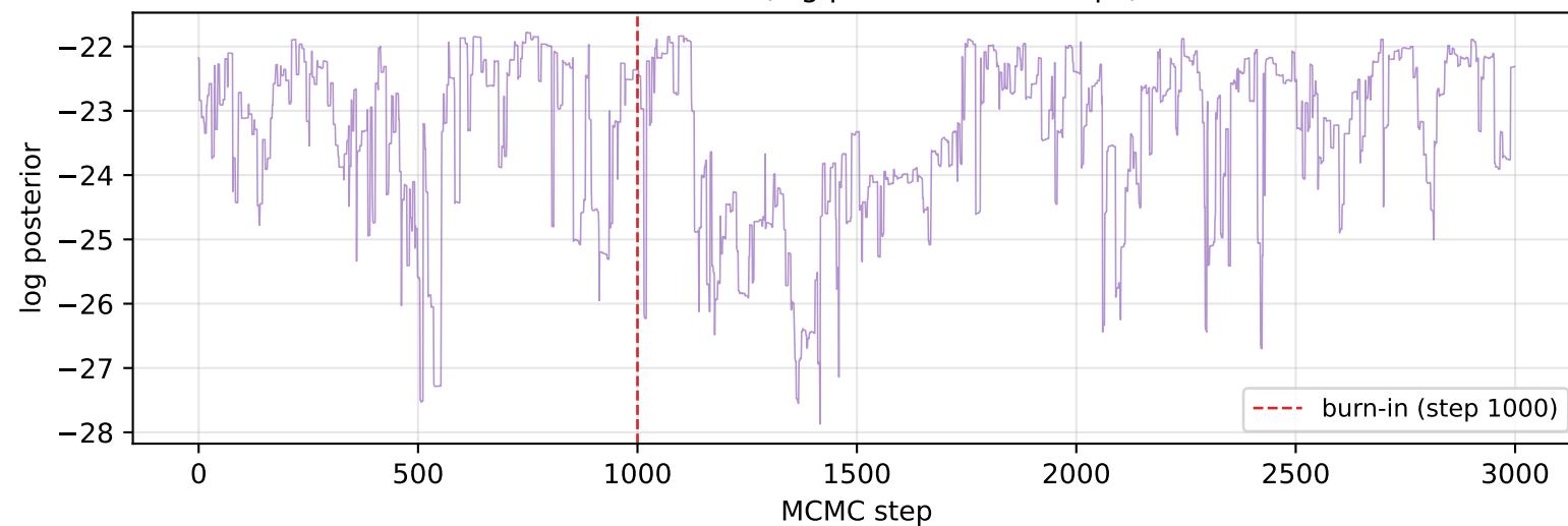
MCMC trace (log posterior over steps)
