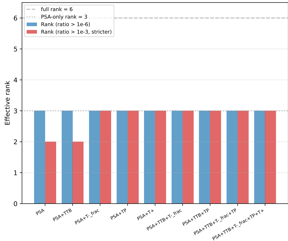
[B] Effective FIM rank vs channel combo
