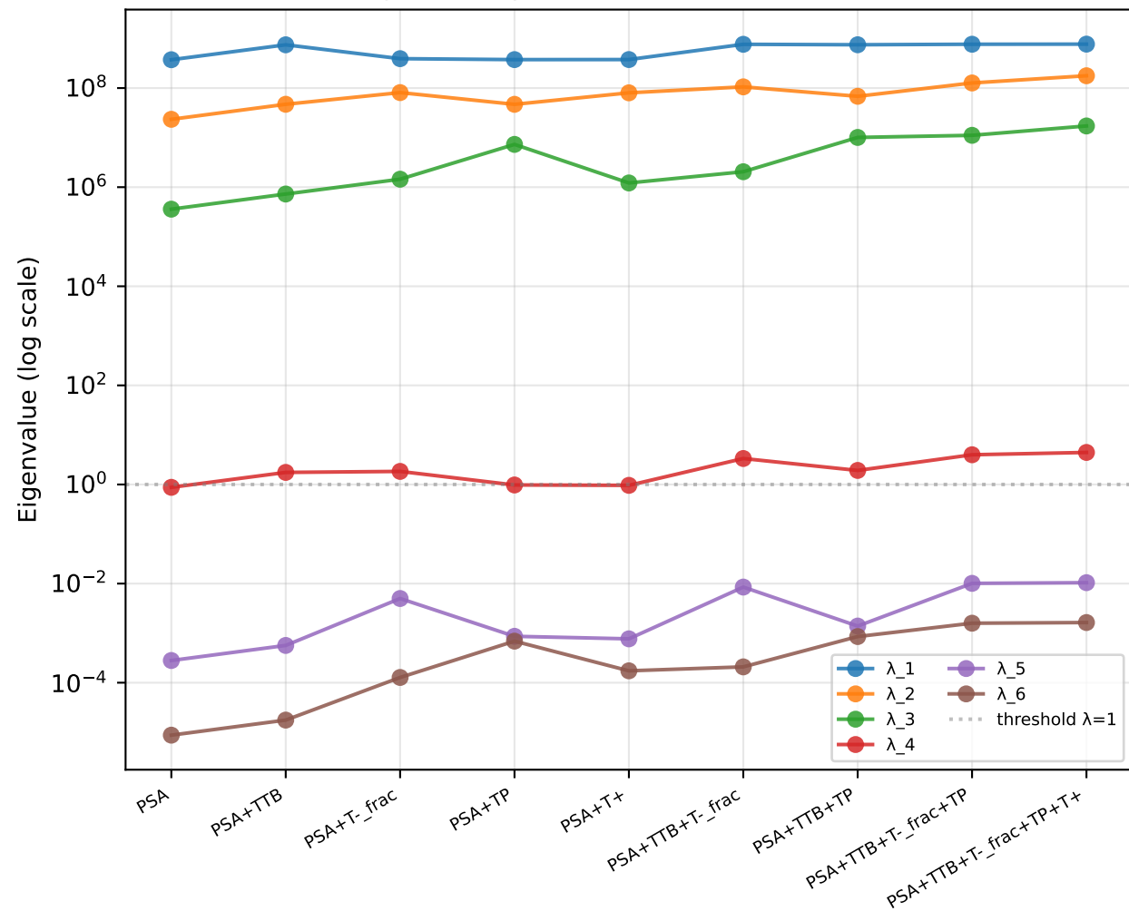
[A] FIM eigenvalue spectrum vs observation channel combo
