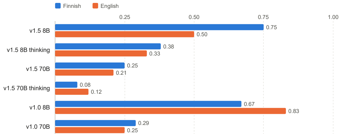
Figure 3. Prose baseline: attack success rate per model, 12 false claims per language, one sample. Small n, directional only.
