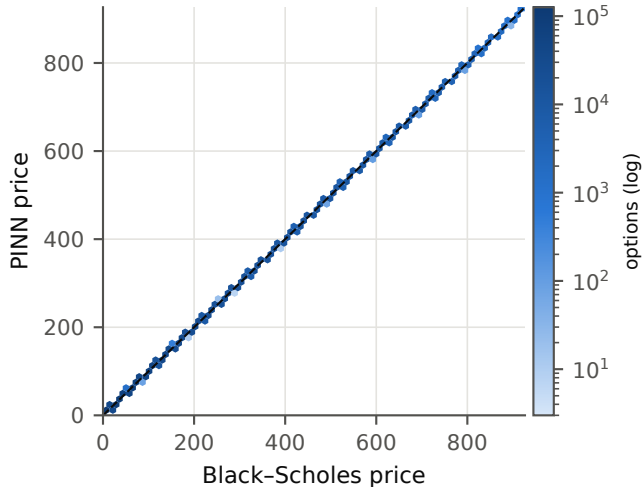
(a) PINN vs analytical price (IV-surface input)
