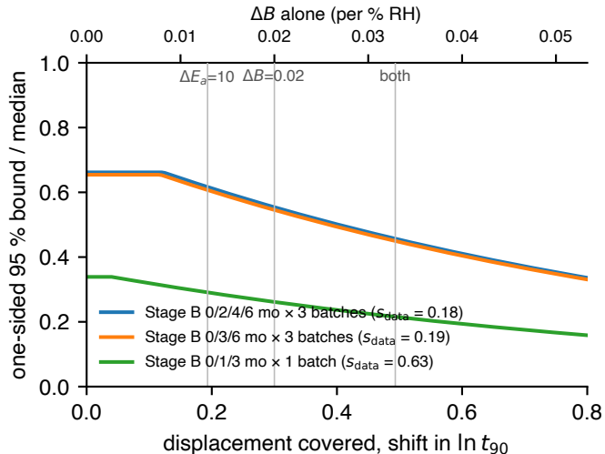
(b) bound after inflating the prior (SD 5, 0.01)
