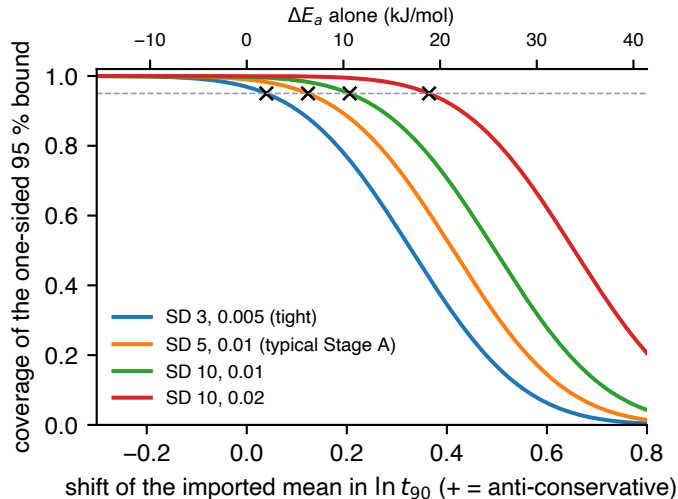
(a) coverage; \times = bias budget
