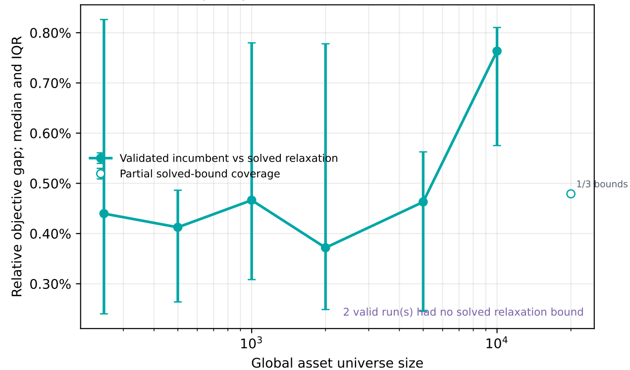
Solution quality (21/21 valid runs had zero breaches)
