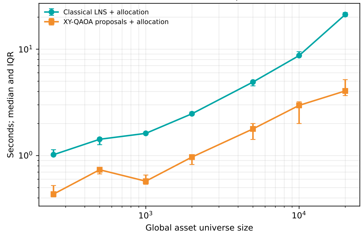
Fixed-window classical and quantum work
