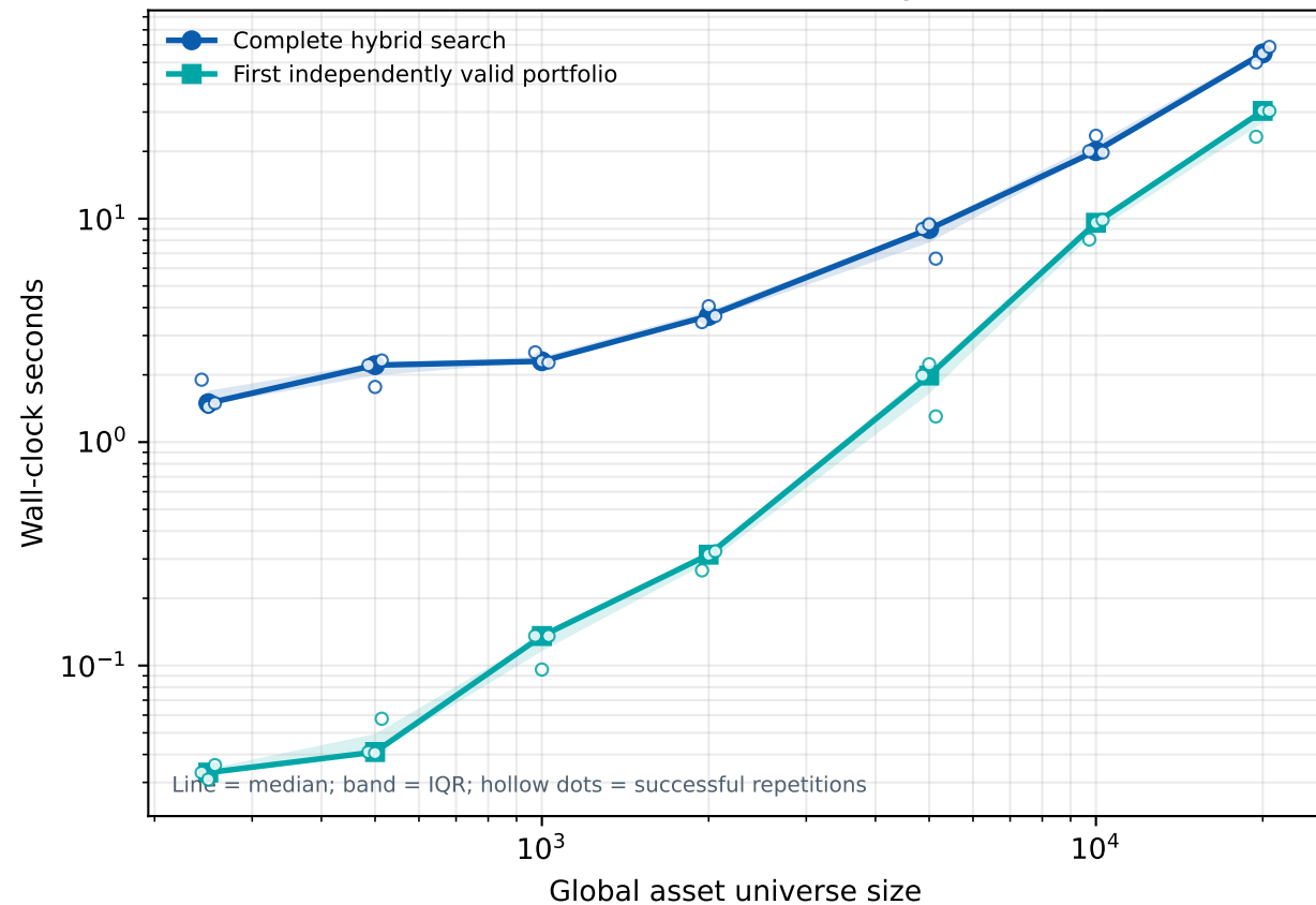
End-to-end scalability
