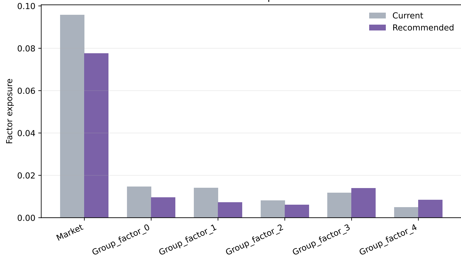
Factor-risk exposure
