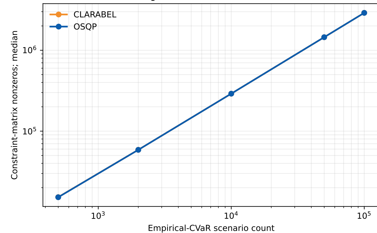
Linear growth of the CVaR formulation
