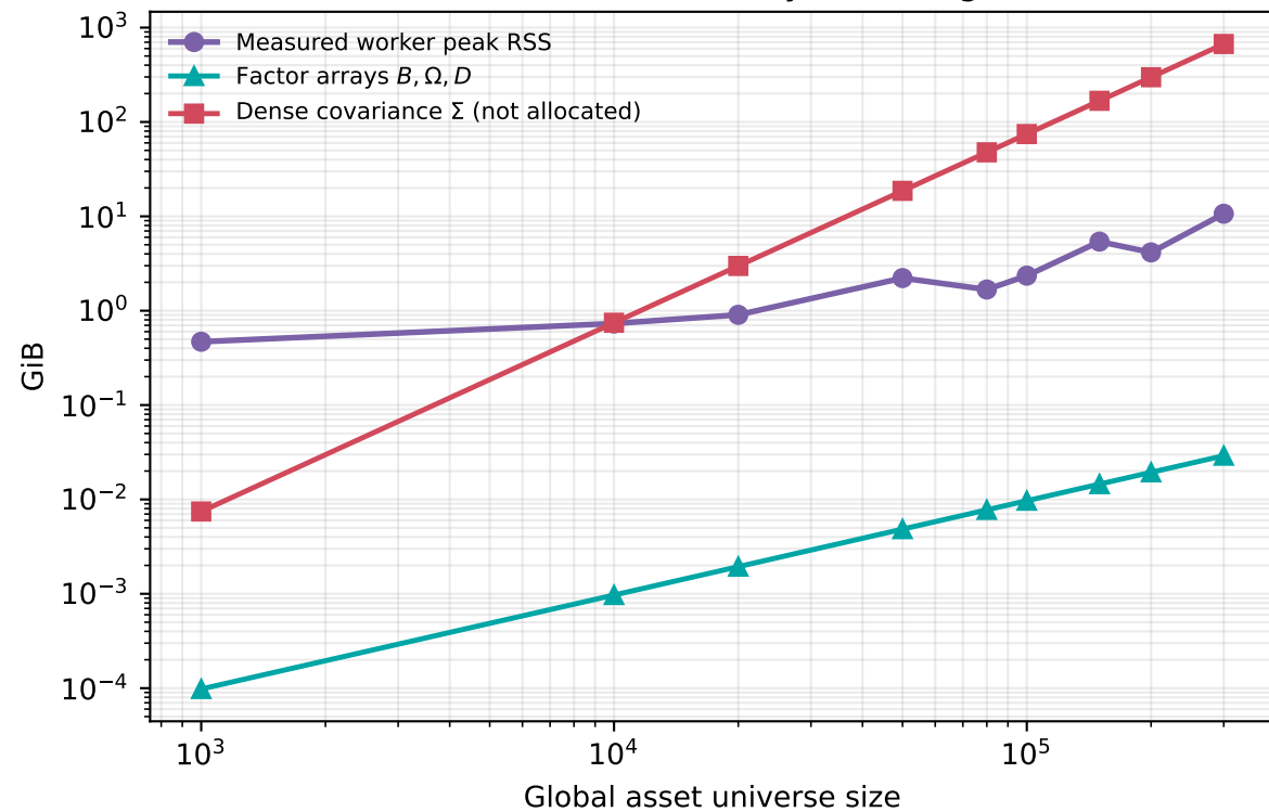
Factor-native memory advantage
