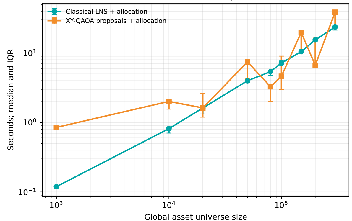
Fixed-window classical and quantum work
