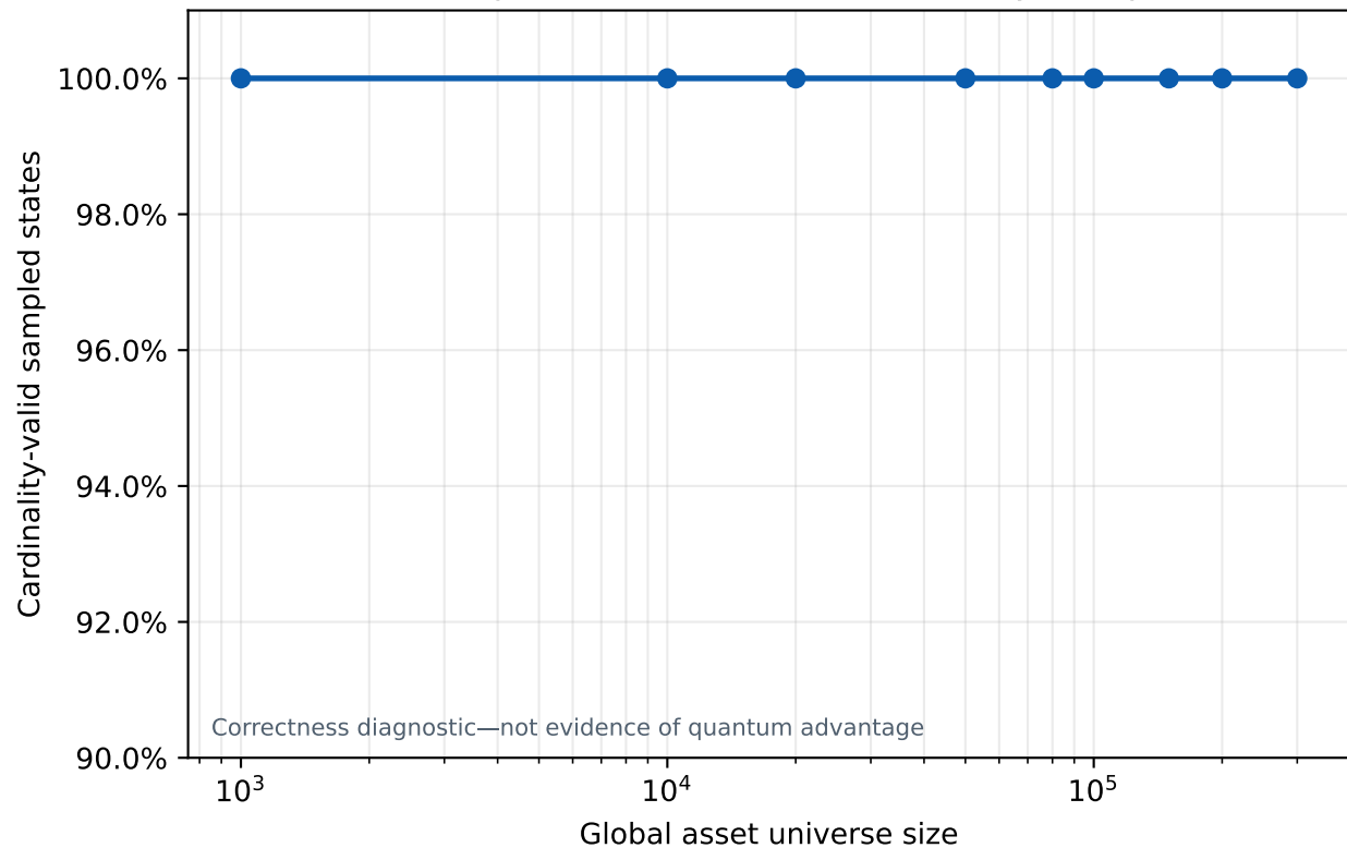
XY mixer preserves the exact-cardinality subspace
