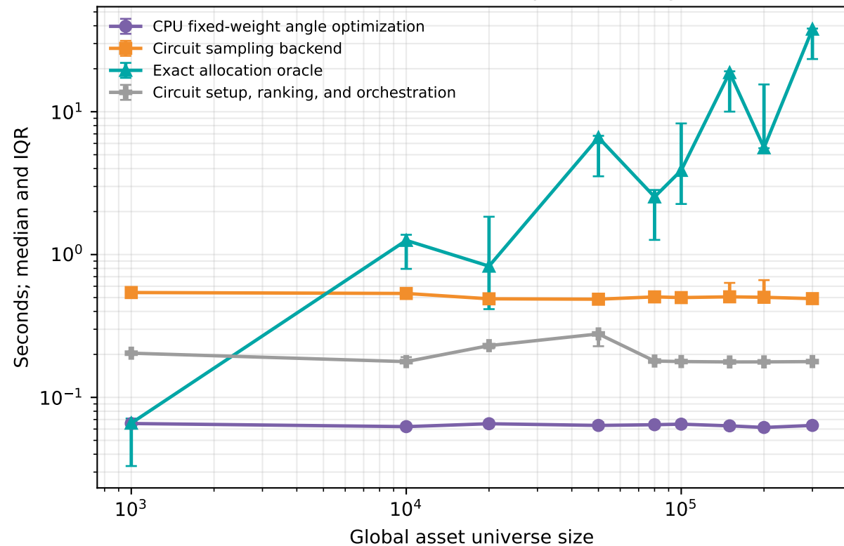
Fixed-window XY-QAOA phase timing
