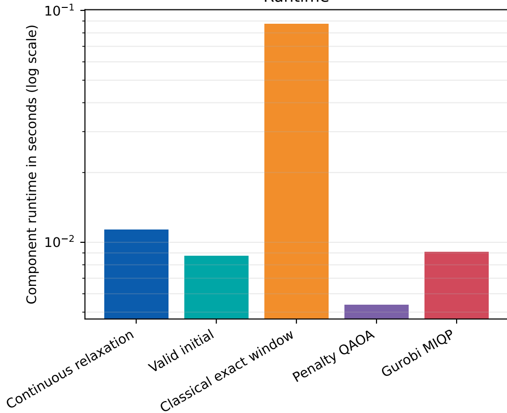
Runtime
