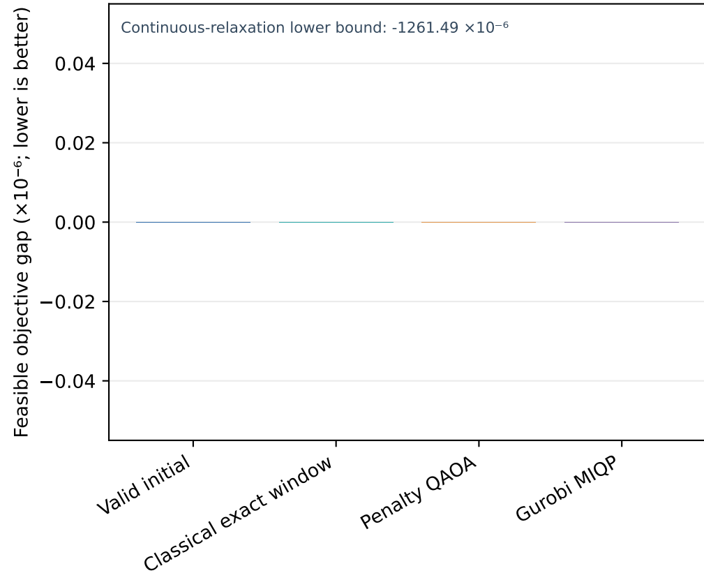
Solution quality
