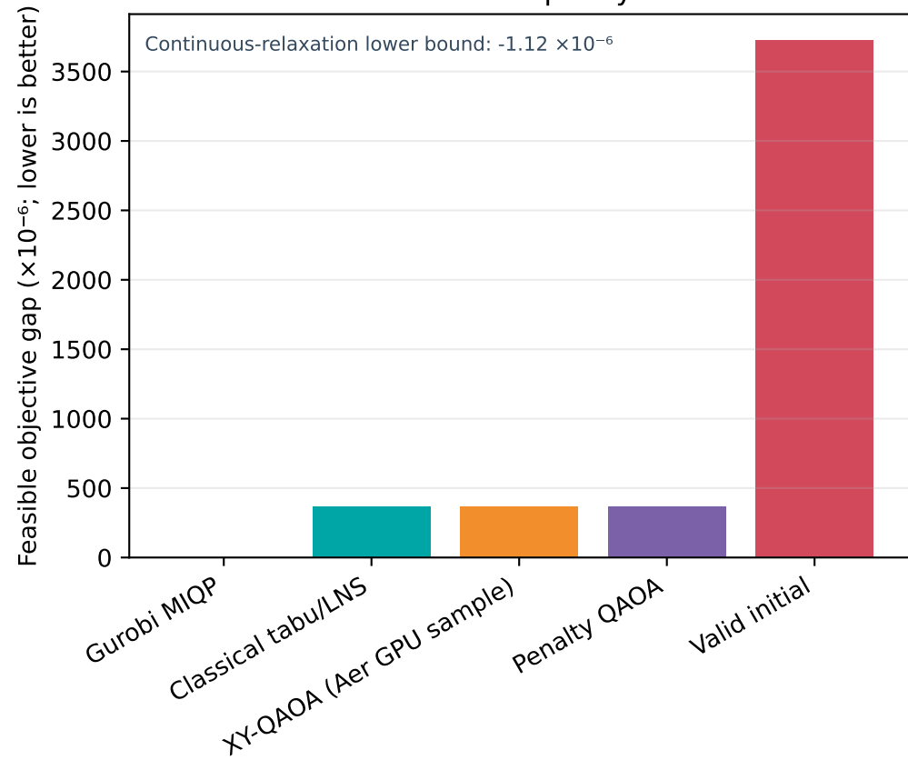
Solution quality
