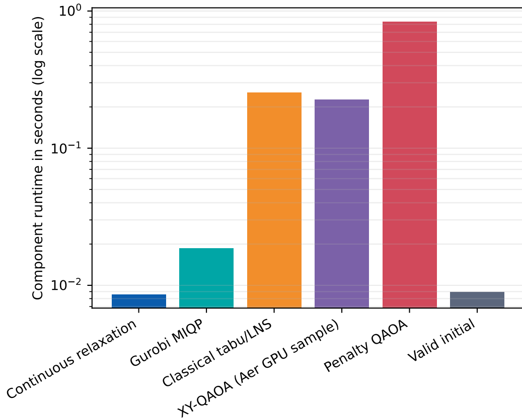
Runtime
