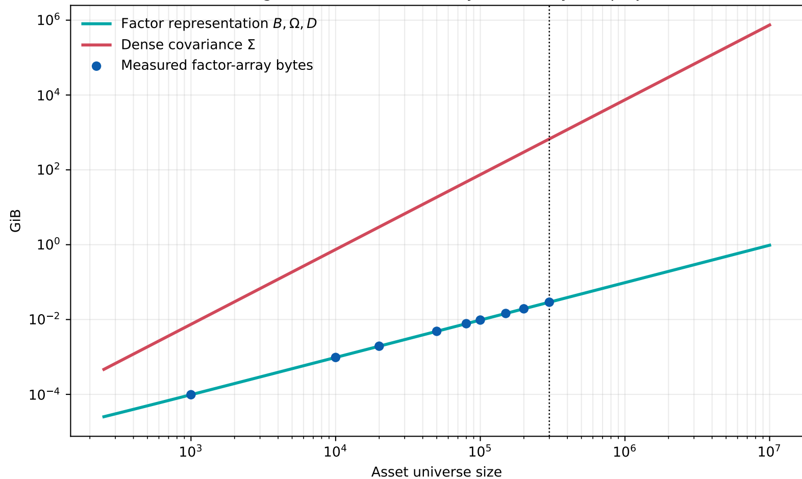
Risk storage: measured factor arrays and analytical projection
