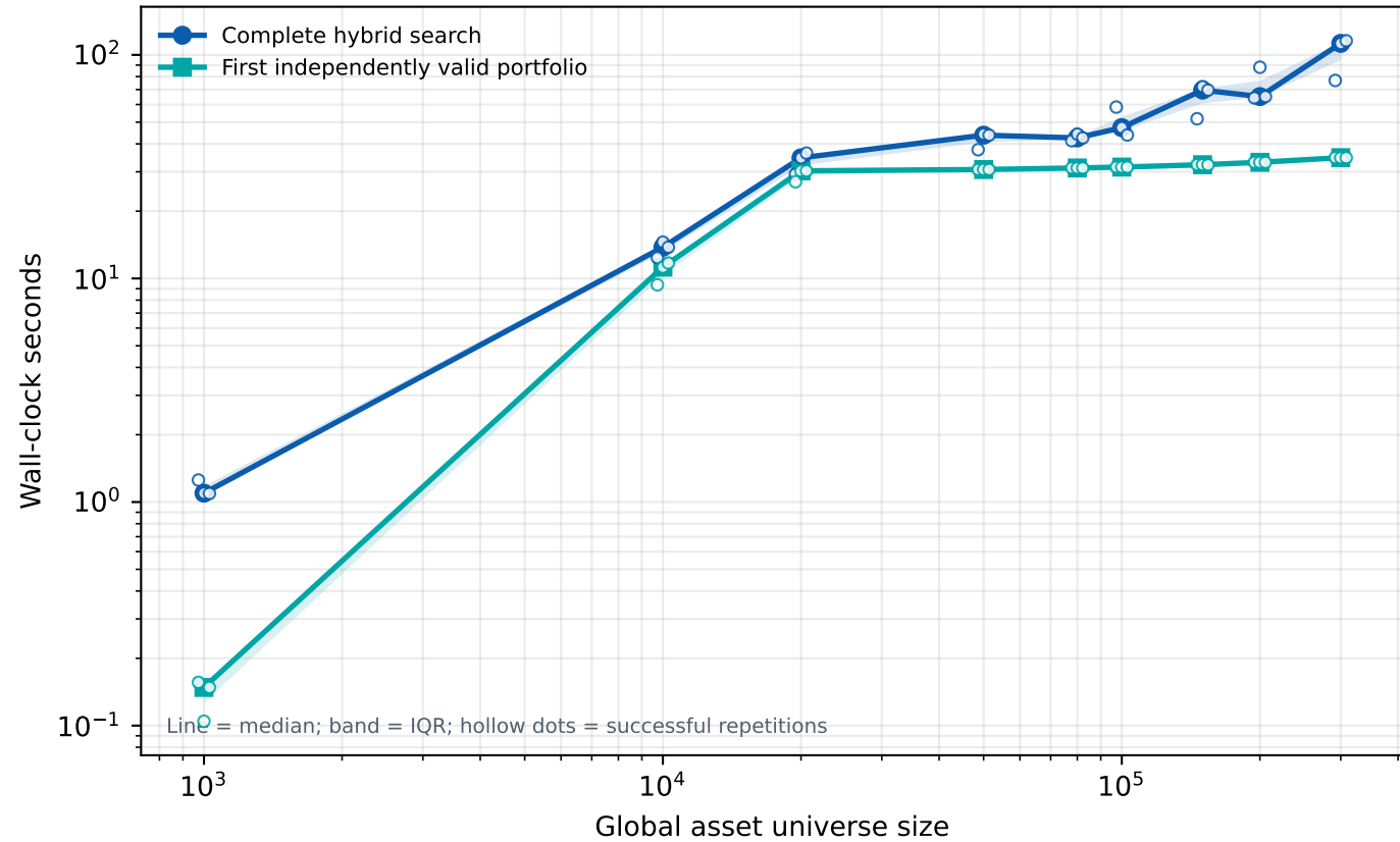
End-to-end scalability
