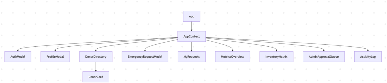
Fig 2: Component Hierarchy
