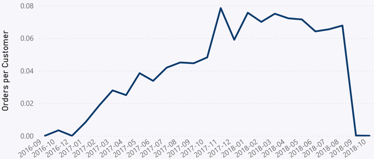
Orders per Customer-Monthly Trend
