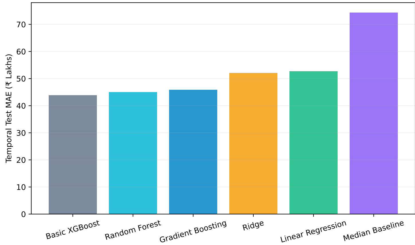
Baseline Model MAE Comparison (Temporal Test Set)
