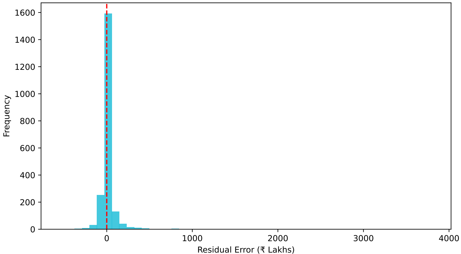
Residual Error Distribution (Basic XGBoost Baseline)
