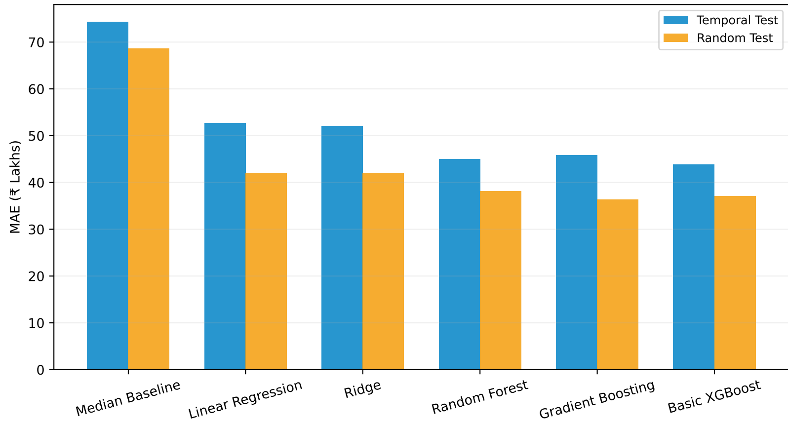
Temporal vs Random Split Performance Comparison (Test Set)
