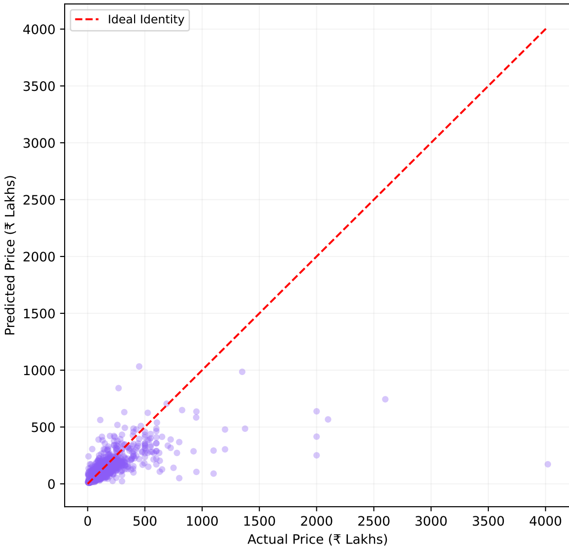
Actual vs Predicted Price (Optimized XGBoost v4)
