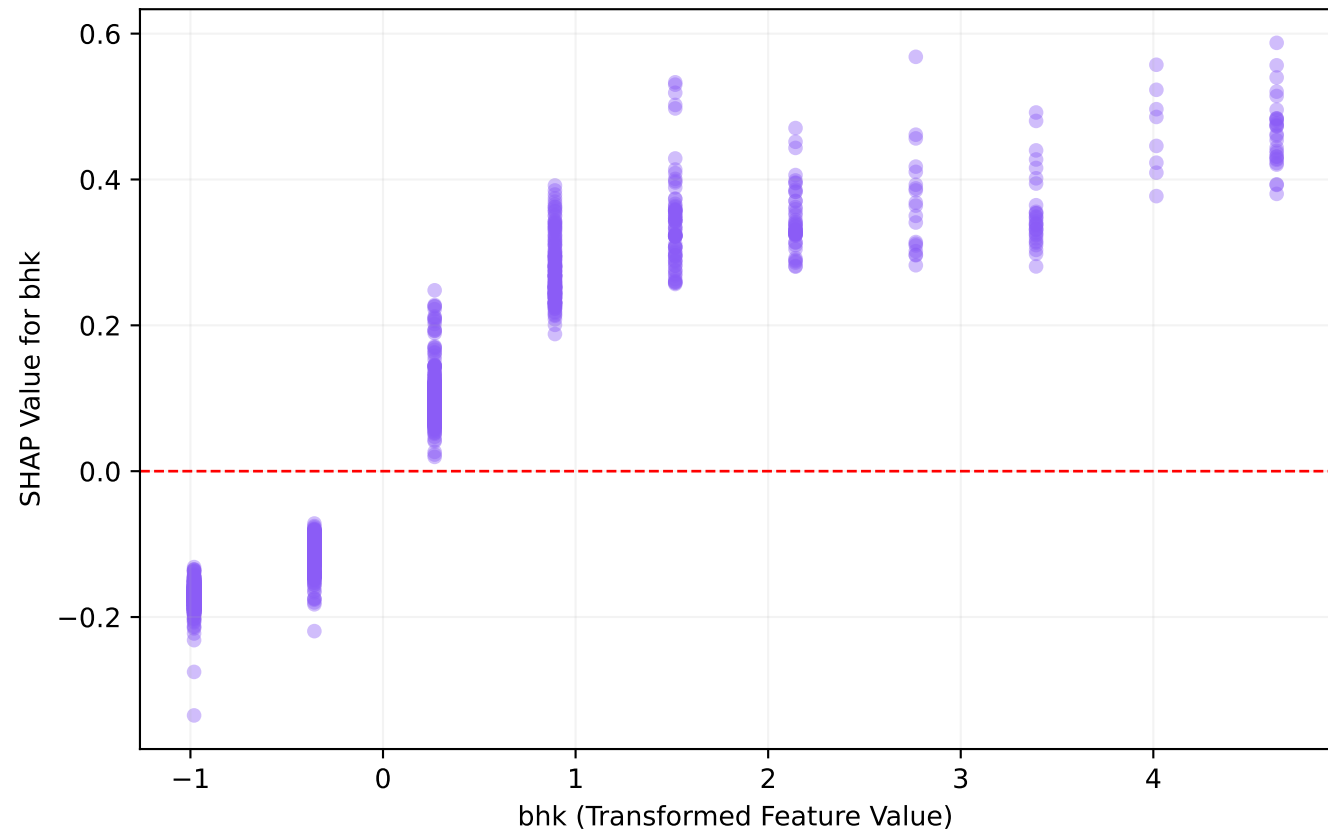
SHAP Dependence Plot: bhk
