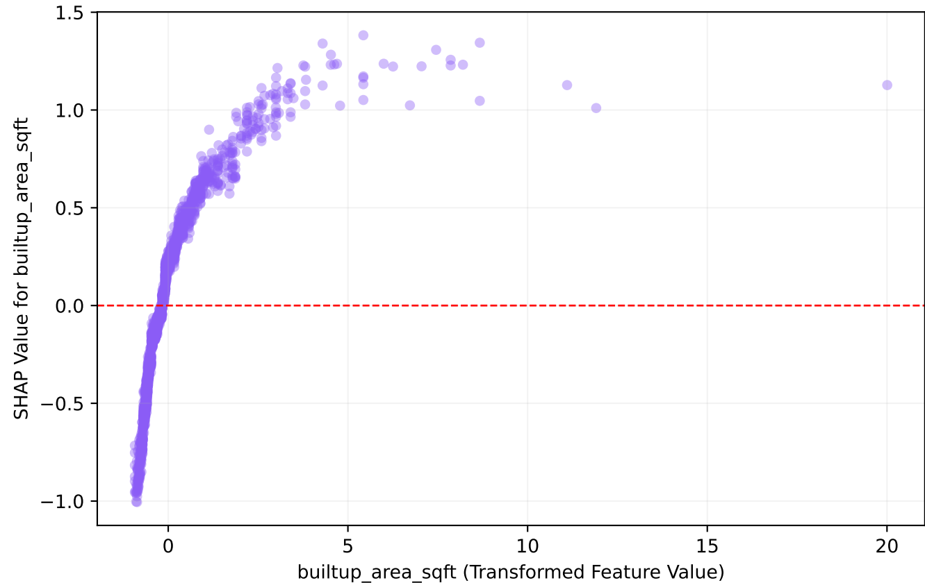
SHAP Dependence Plot: buildup_area_sqft
