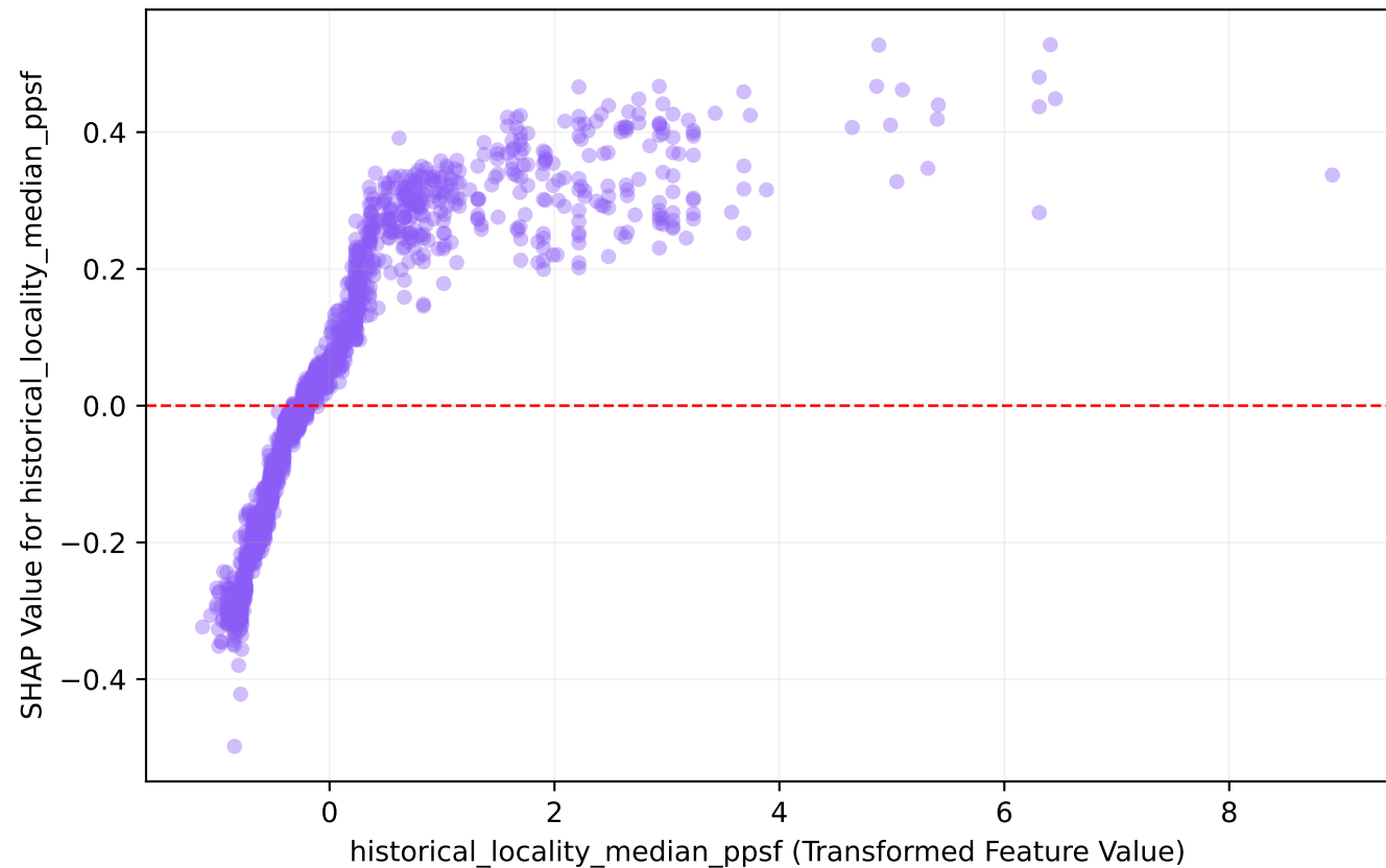
SHAP Dependence Plot: historical_locality_median_ppsf
