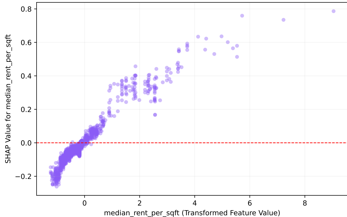
SHAP Dependence Plot: median_rent_per_sqft
