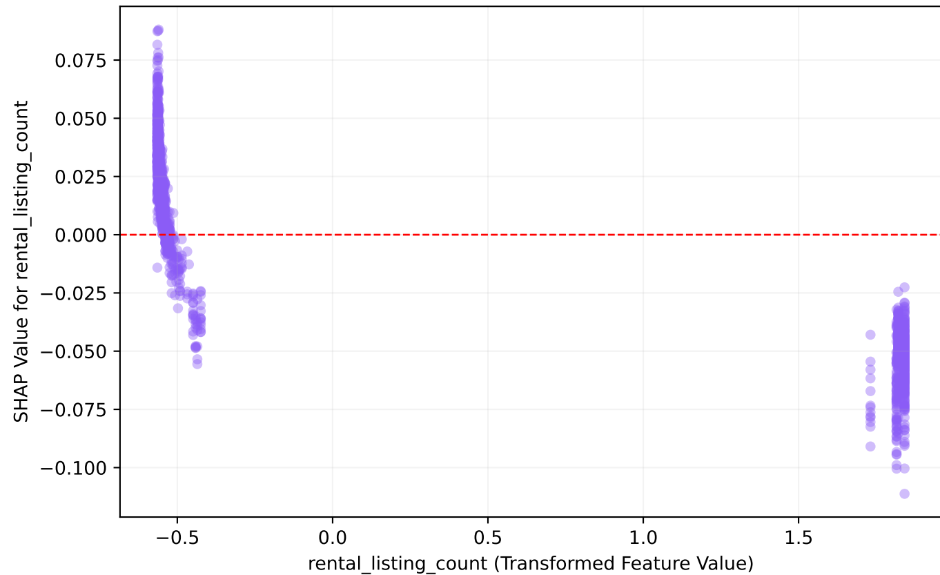
SHAP Dependence Plot: rental_listing_count
