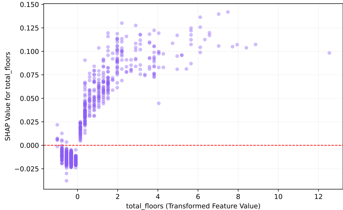
SHAP Dependence Plot: total_floors
